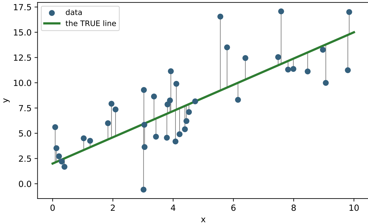
Even the true line misses each point (natural noise)
