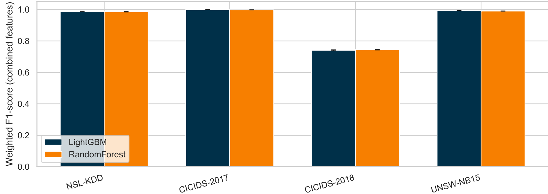
LightGBM vs Random Forest — Combined MDE Feature Set
