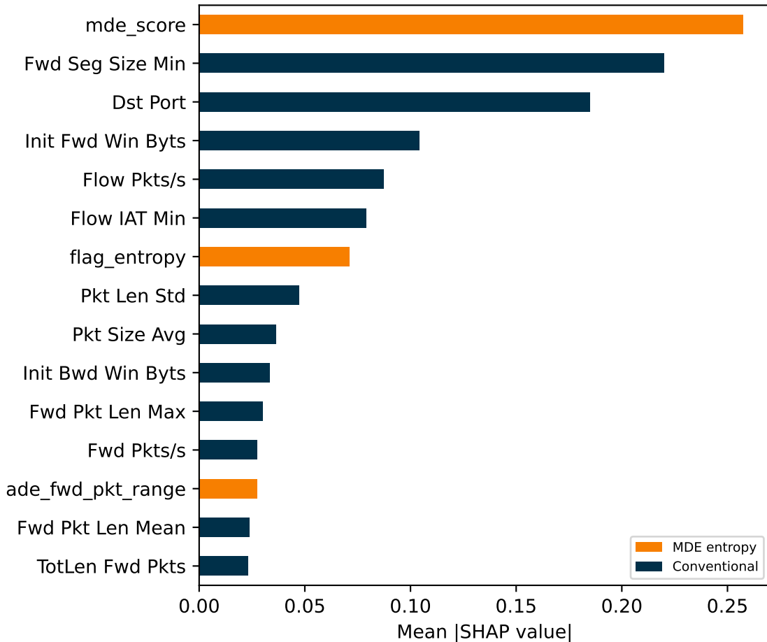
SHAP Importance — CICIDS-2018
