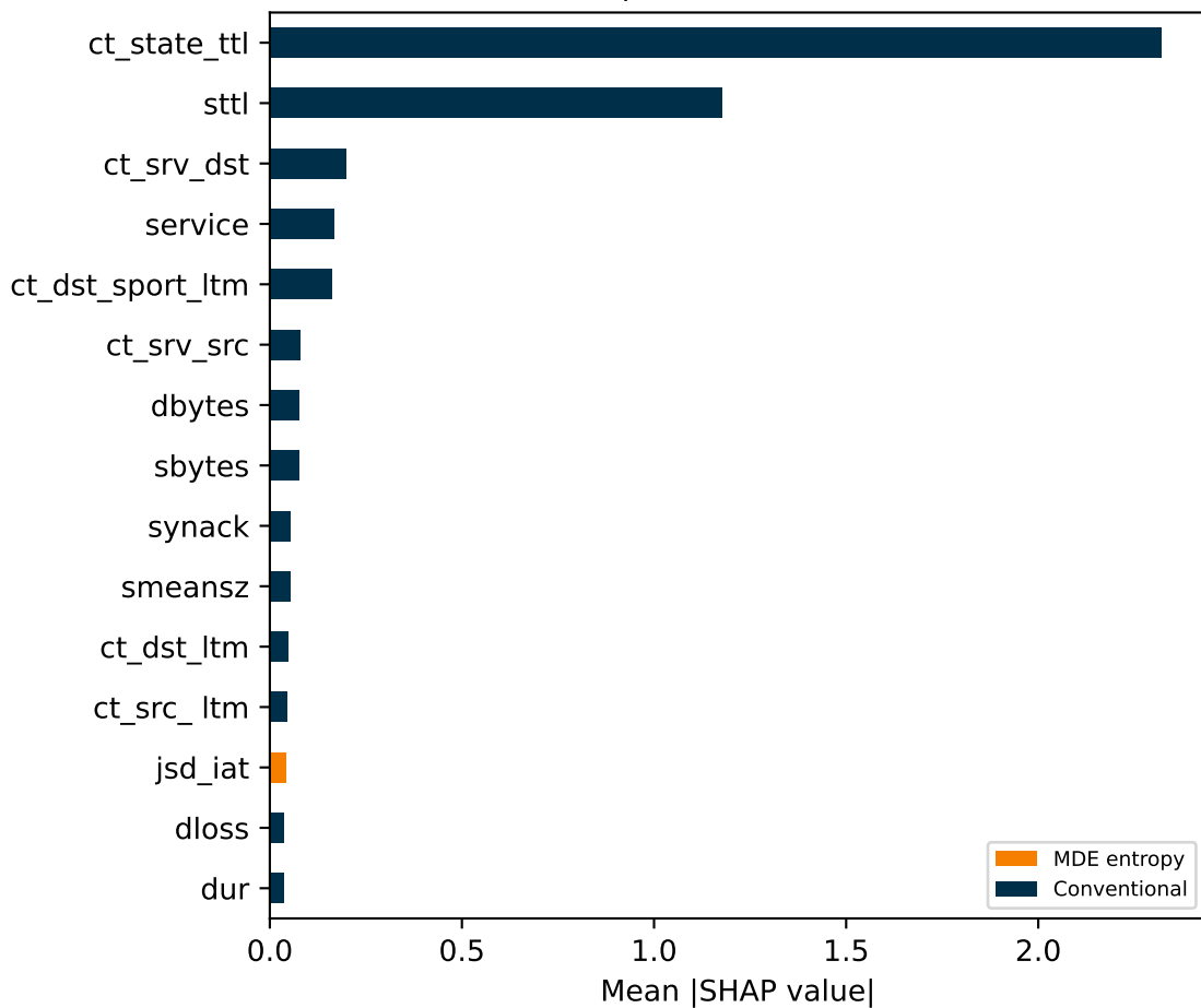
SHAP Importance — UNSW-NB15
