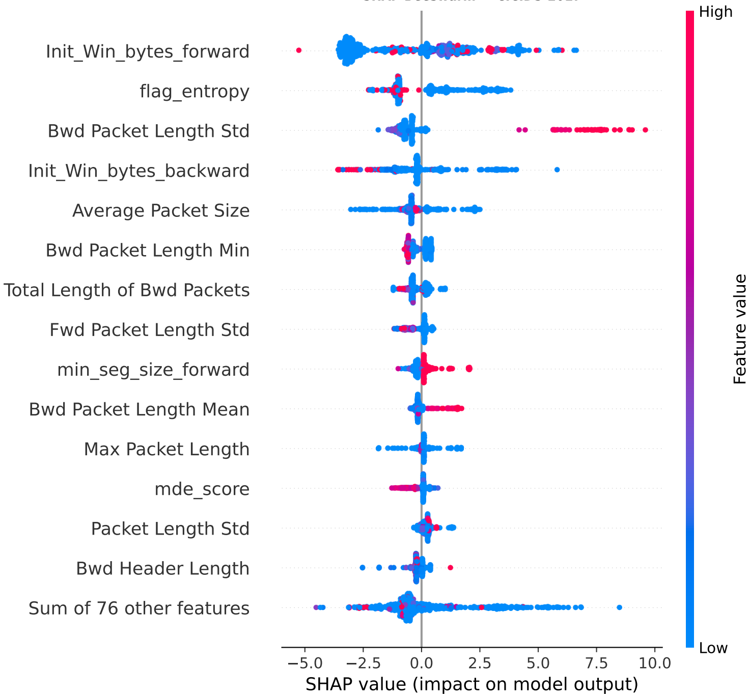
SHAP Beeswarm — CICIDS-2017
