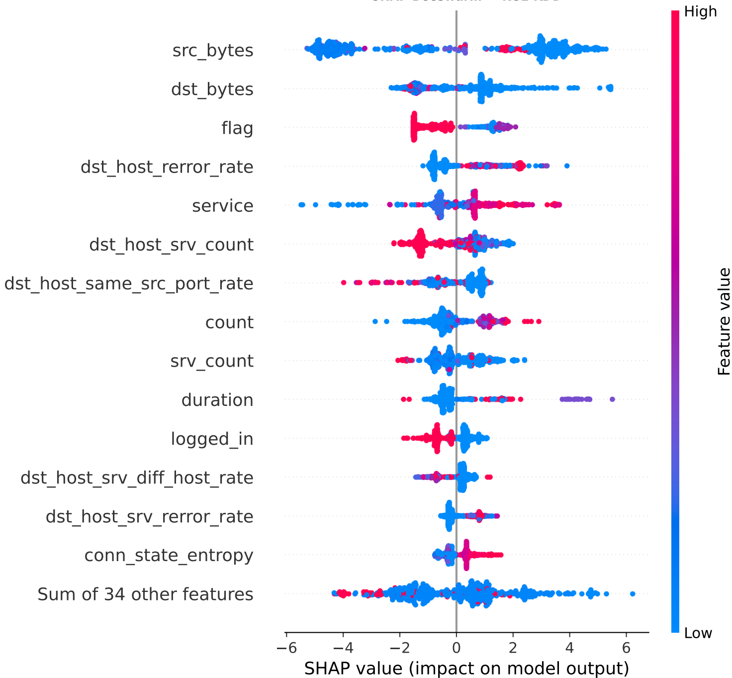
SHAP Beeswarm — NSL-KDD
