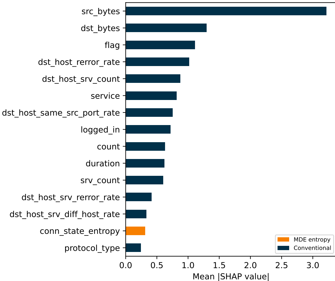
SHAP Importance — NSL-KDD
