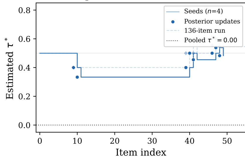
(c) Empirical: Haiku 4.5 (50 items)
