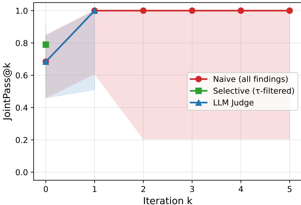
Joint Functional + Security Pass Rate
