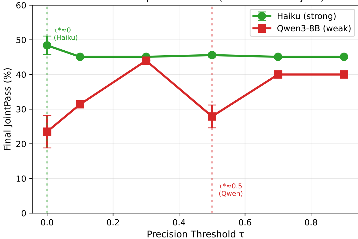
Threshold Sweep on 51 Items (Combined Analyzer)
