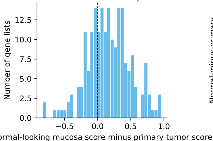
A: Gene-list score comparison
