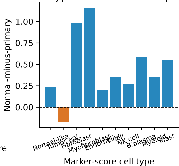
B: Cell-type marker-score comparison
