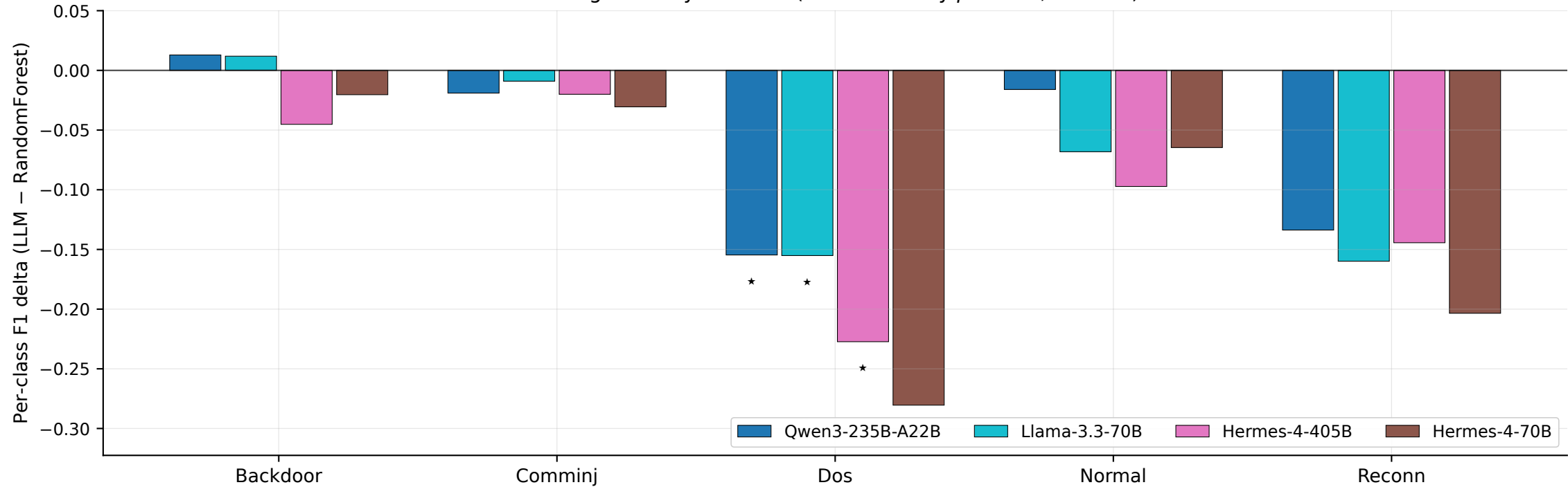
WUSTL multi-class: per-class F1 deltas relative to RandomForest
