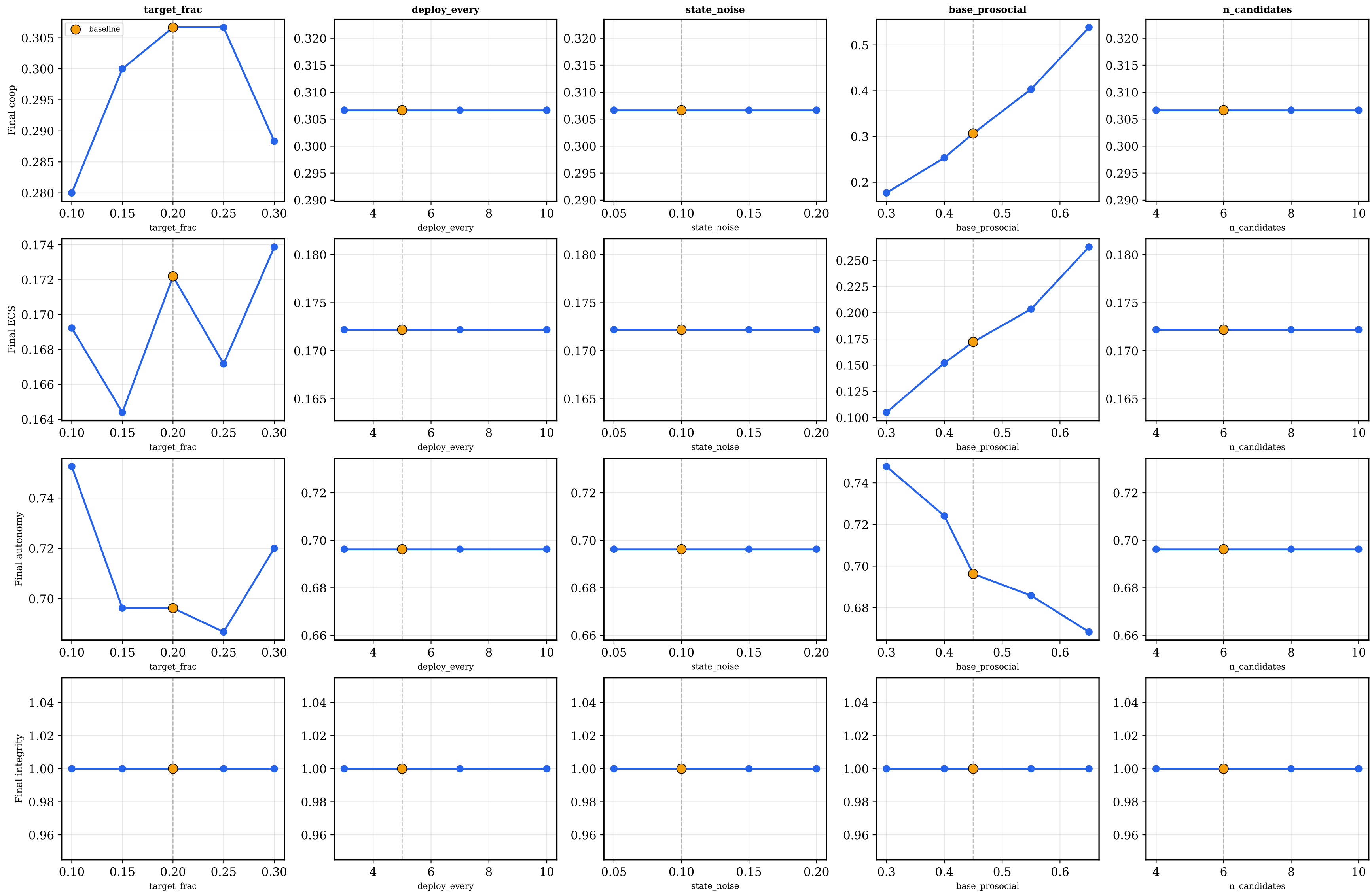
R3 OAT Sensitivity -- GCGE governed adversarial (scale-free, n=30, seed=42)
