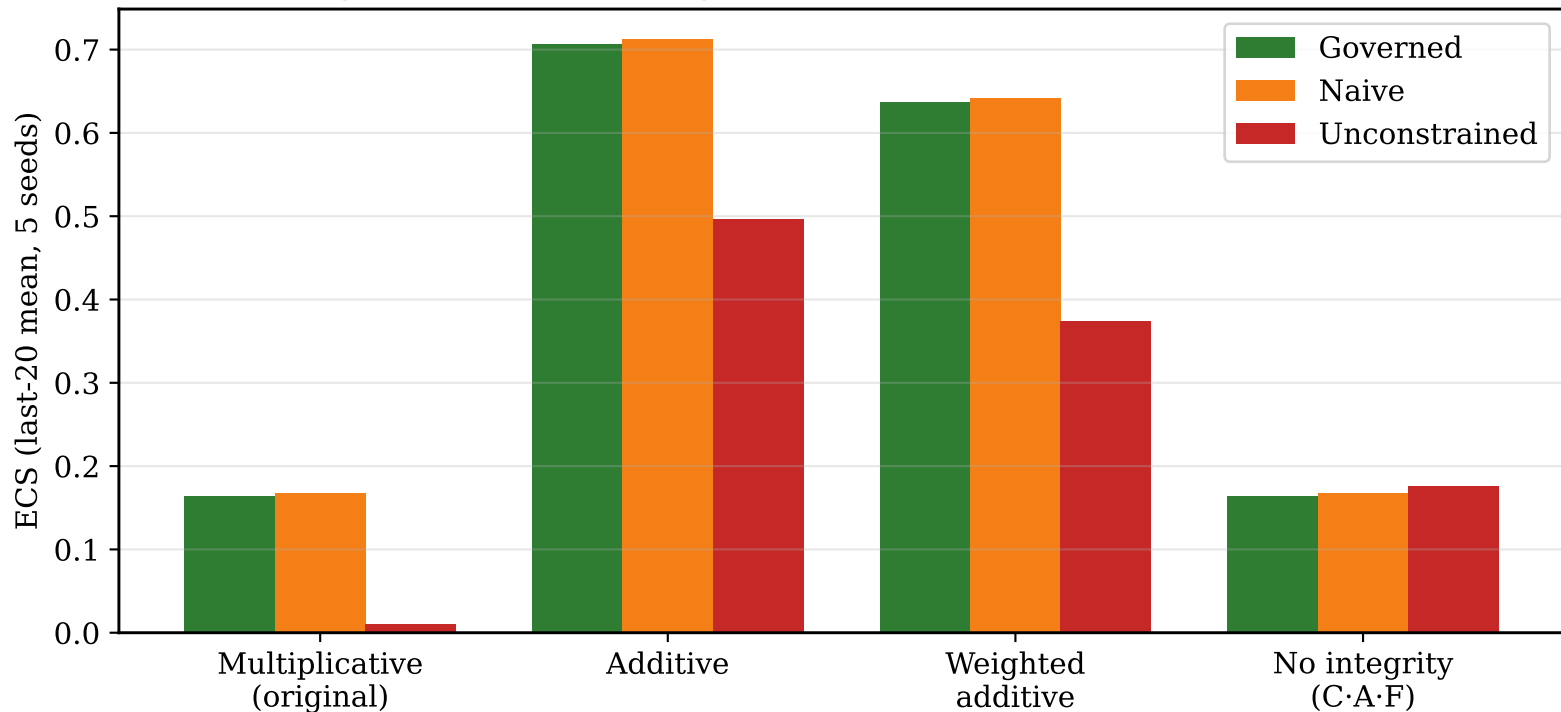
ECS governance advantage under alternative metric formulations
