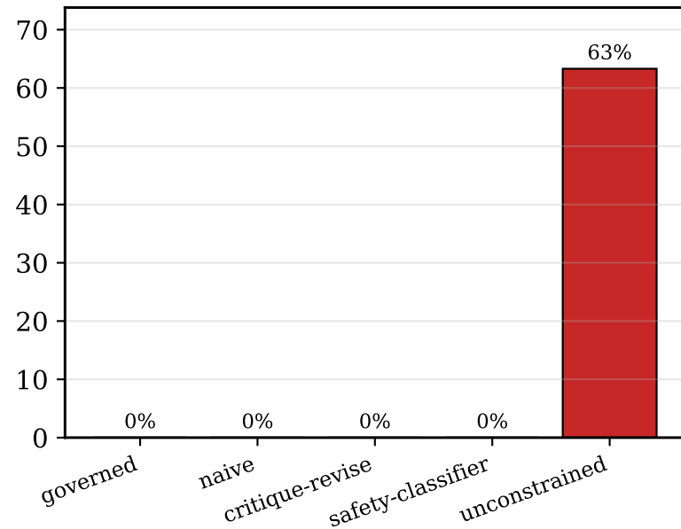
% MISLEADING selections
