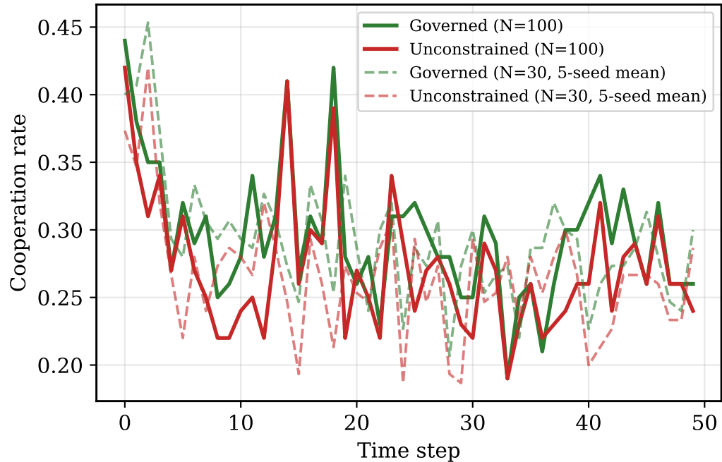
Cooperation rate at N=100 vs. N=30 baseline
