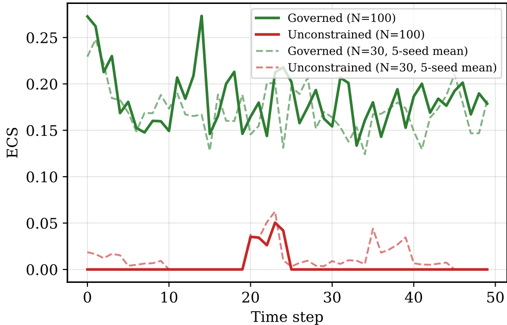
ECS at N=100 vs. N=30 baseline
