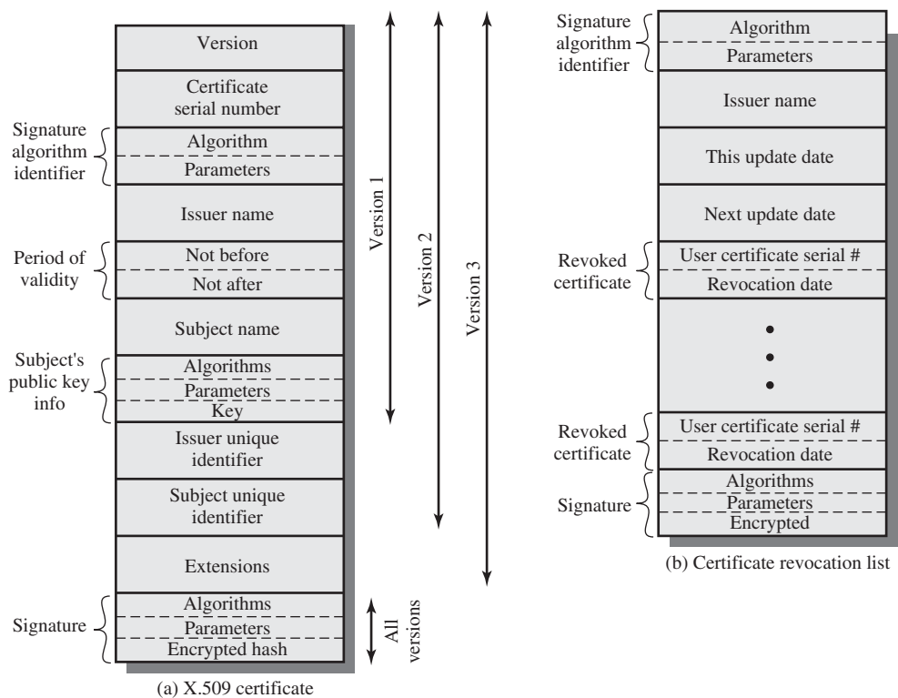
Figure 4.4 X.509 Formats
