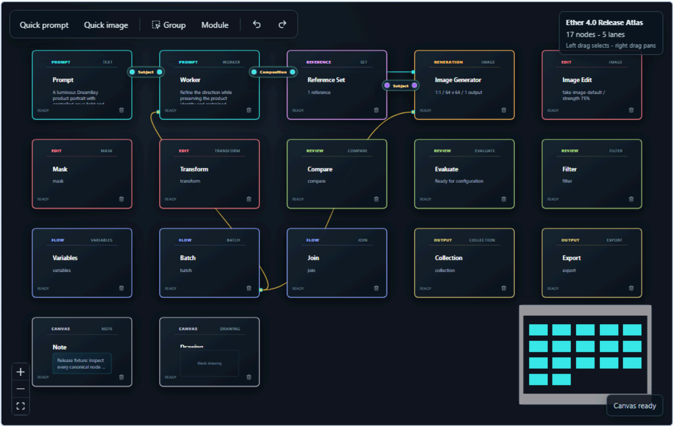
Packaged Ether release capture - Canvas containing all 17 canonical nodes
