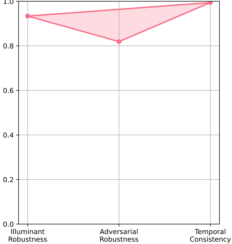
Robustness Scores
