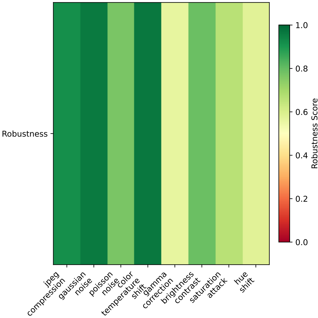
Adversarial Robustness
