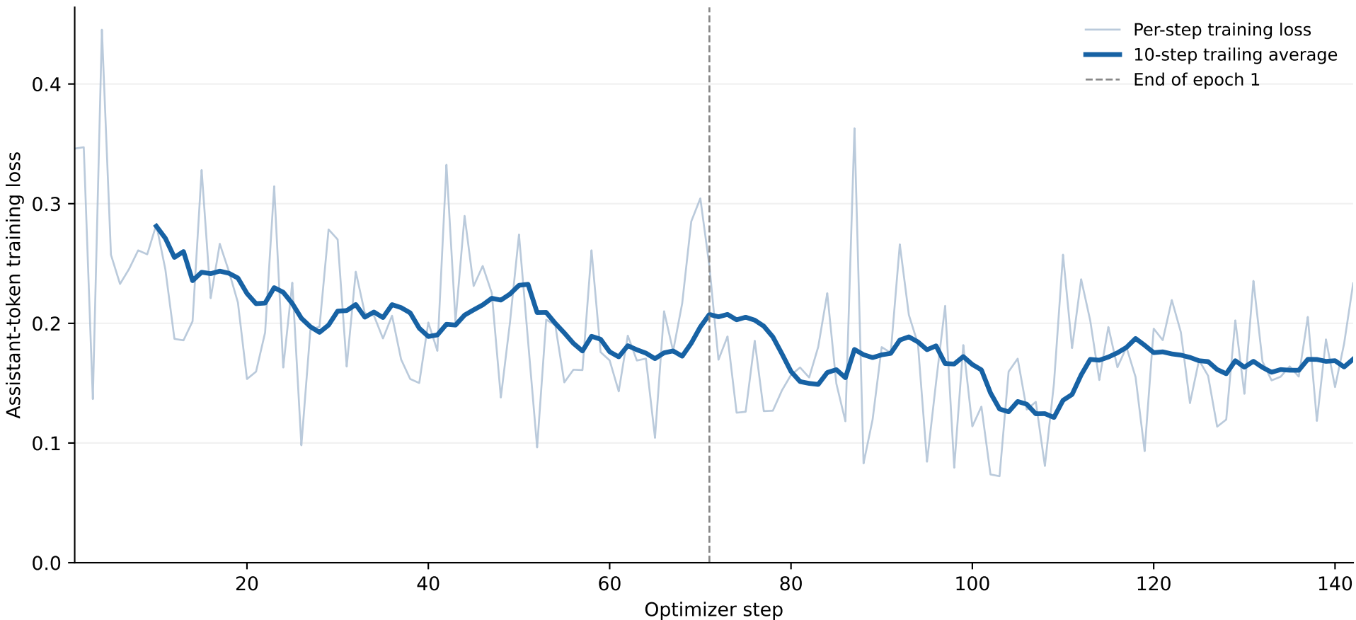
Qwen3.5-4B · FinanceBench QLoRA SFT
