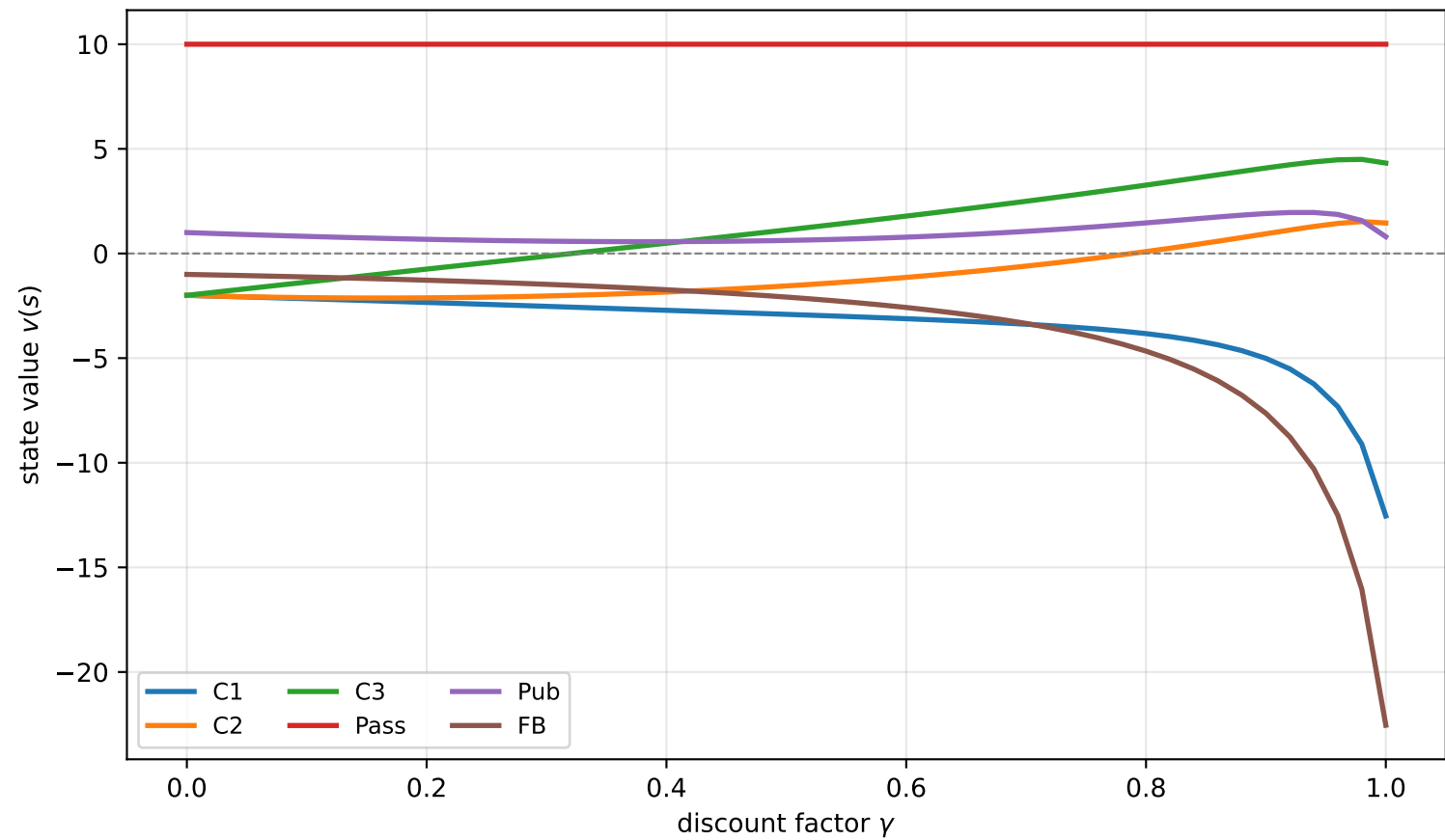
Student MRP: value function vs. discount factor
