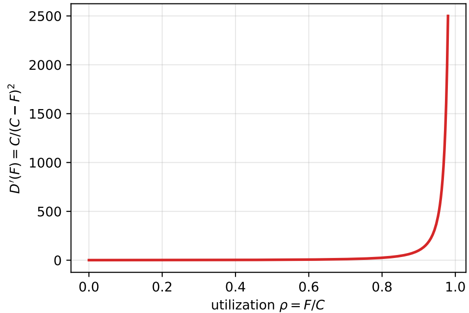
Marginal delay (per-link DFDL term)
