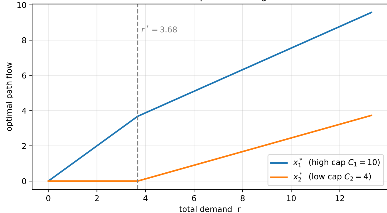
Two-link optimal routing
