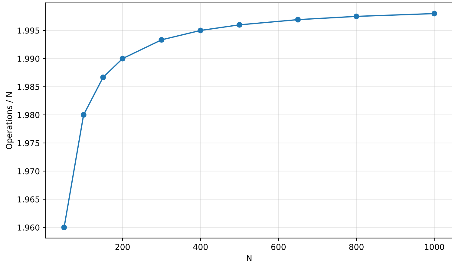
Insertion Sort on already sorted arrays
