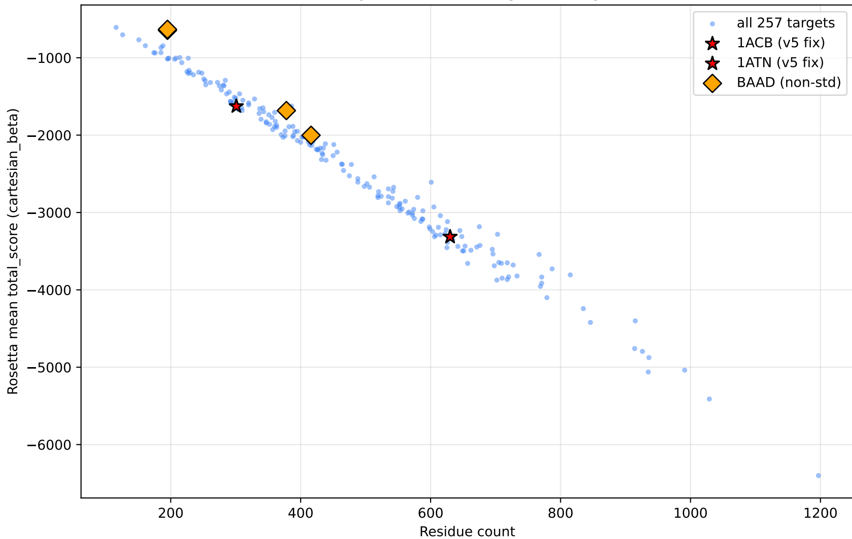
AMBER-crystal Rosetta energies vs target size
