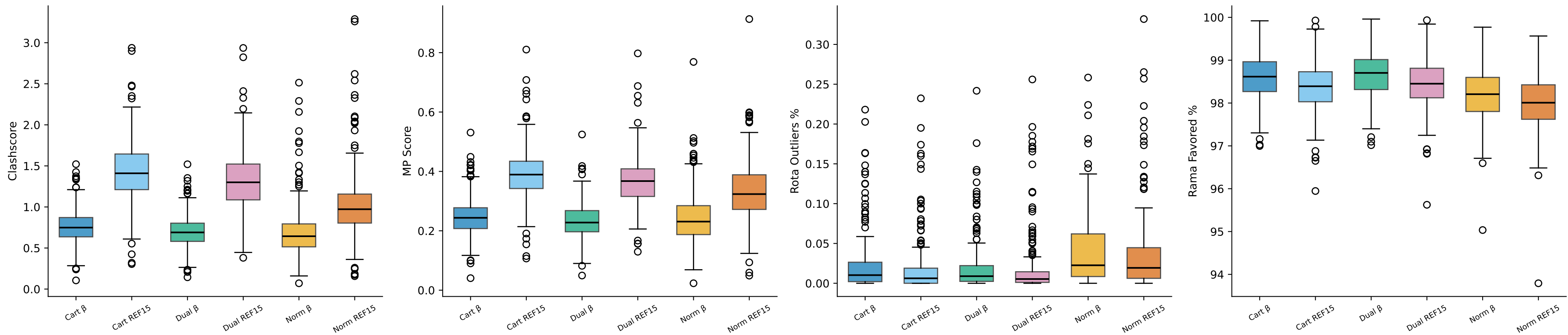
Rosetta Protocol MolProbity Comparison (Green pipeline, per-target averages)
