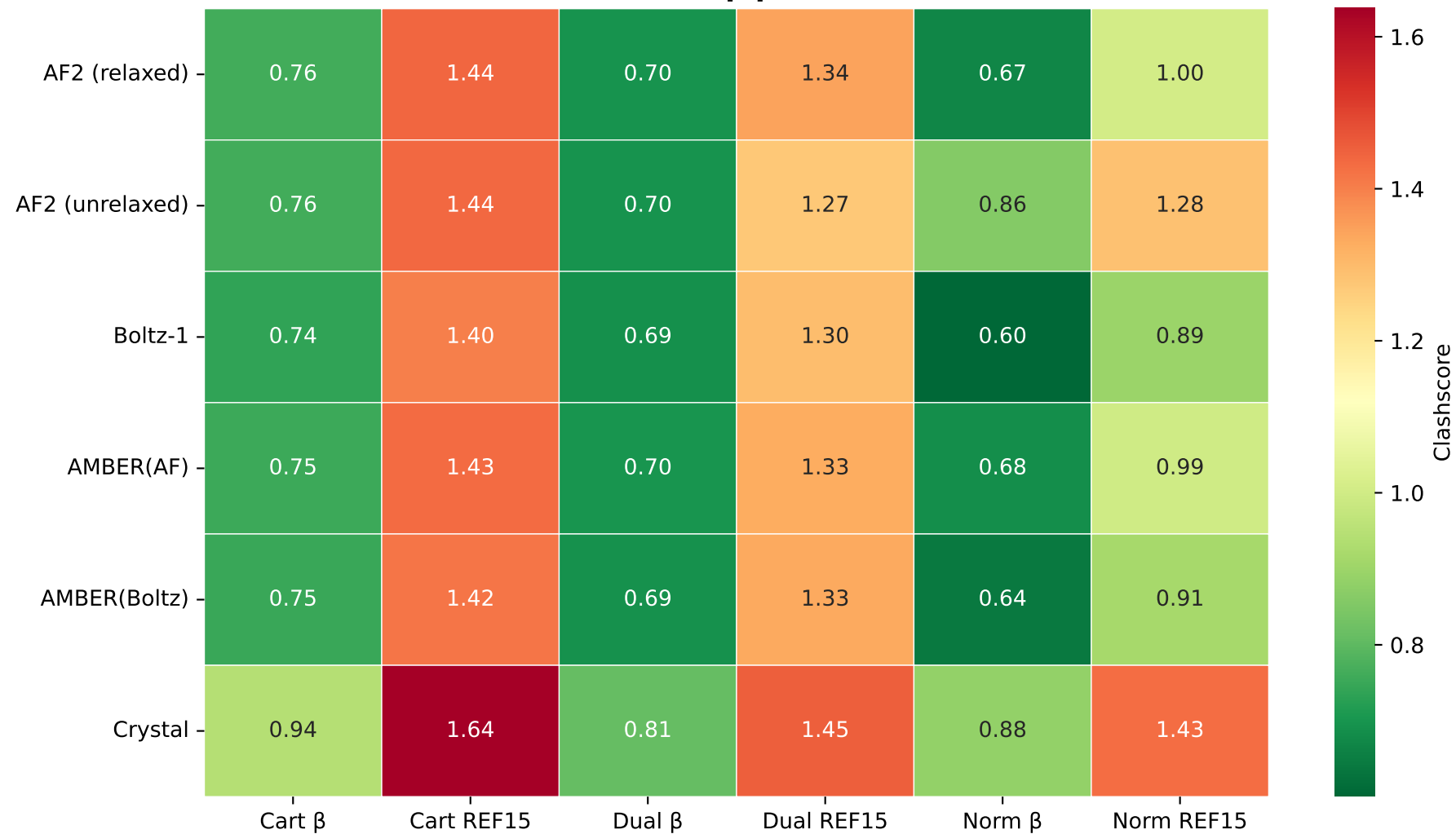
Rosetta Clashscore by Protocol × Source (Green pipeline)
