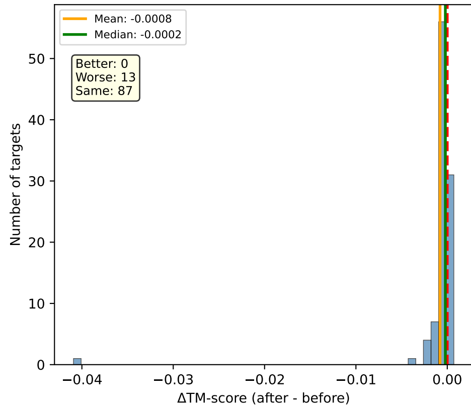
AF2: Built-in AMBER
