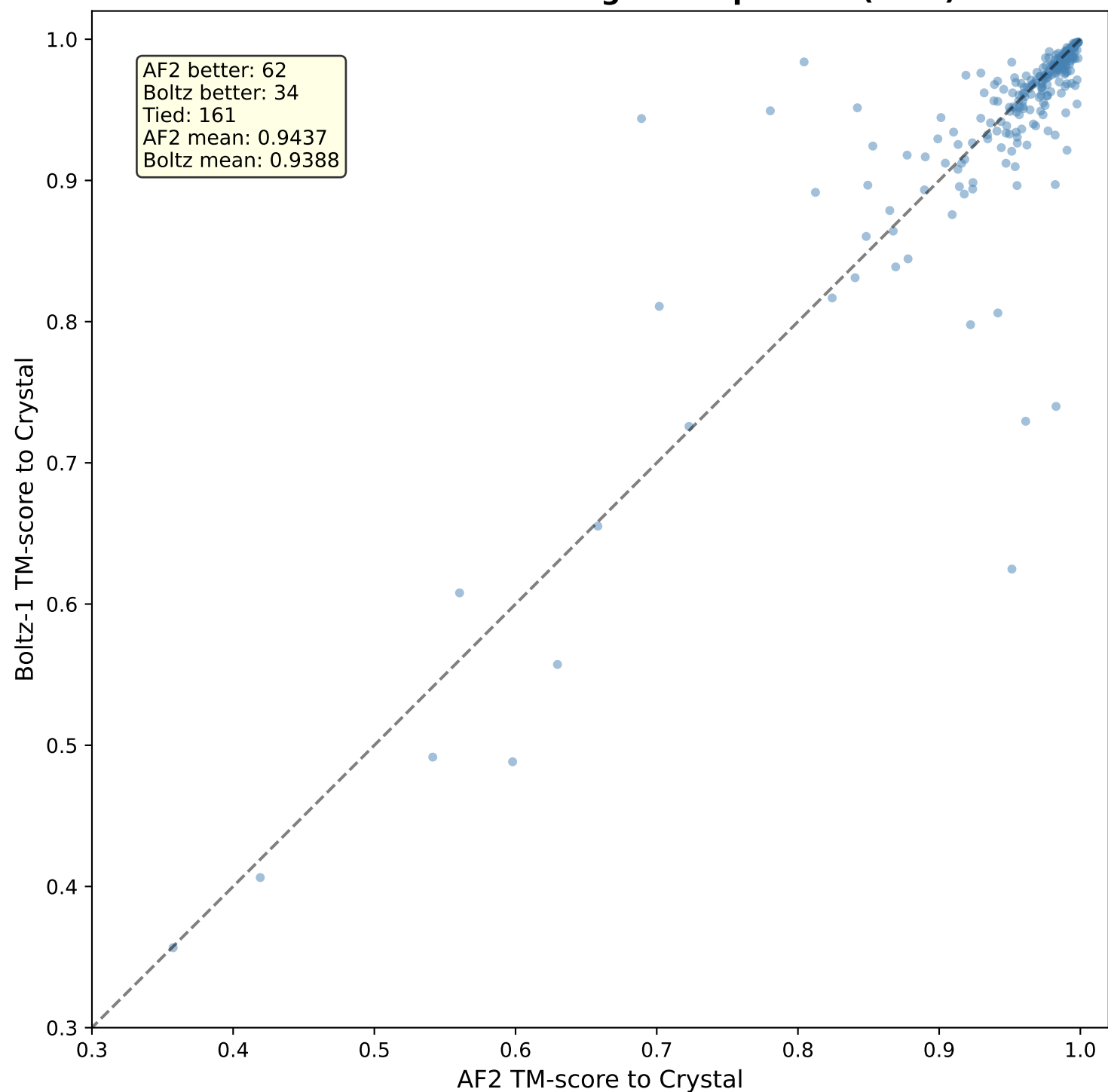
AF2 vs Boltz-1: Per-Target Comparison (Blue)
