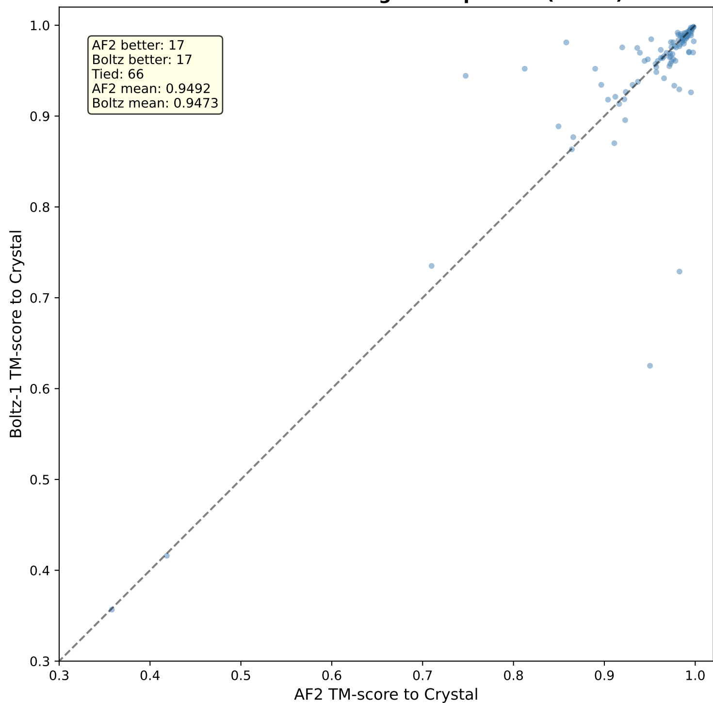
AF2 vs Boltz-1: Per-Target Comparison (Green)
