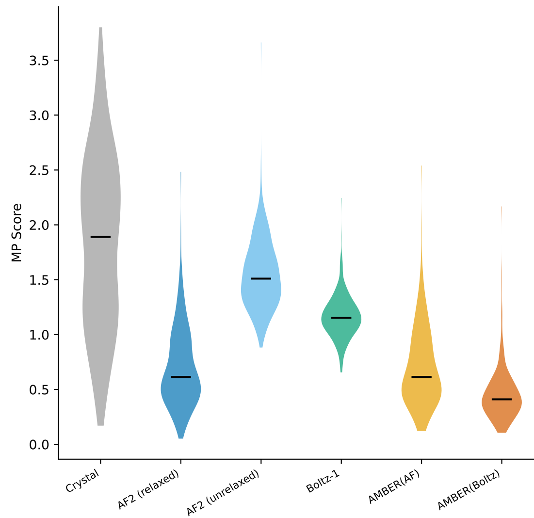
MolProbity Metric Distributions by Source (Green pipeline, per-target averages)
