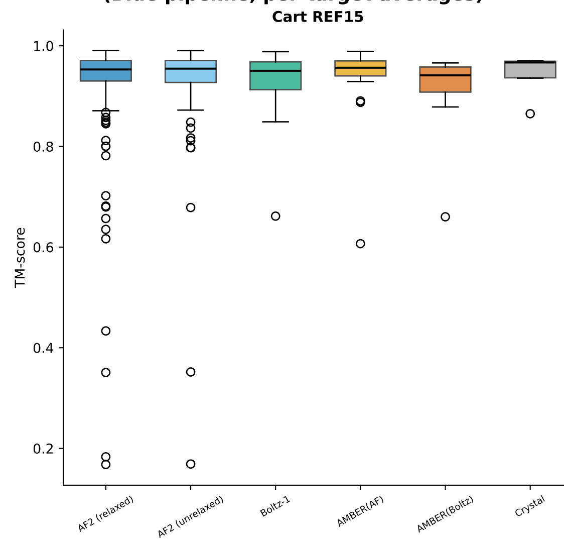
Rosetta TM-score by Input Type (Blue pipeline, per-target averages)
