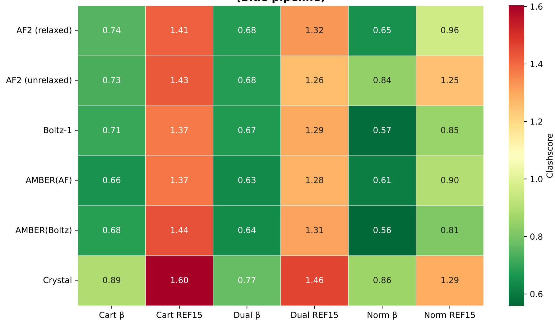
Rosetta Clashscore by Protocol × Source (Blue pipeline)
