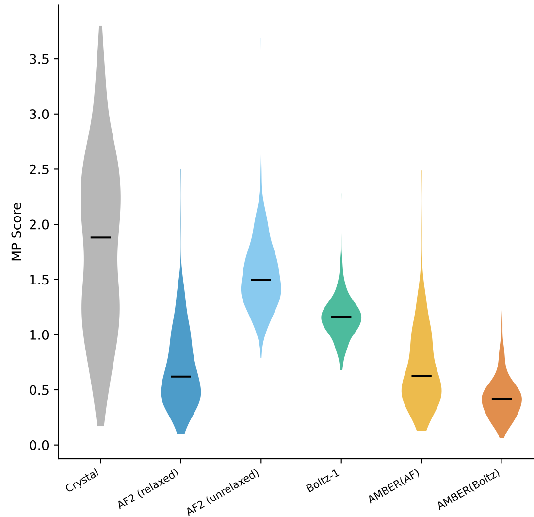
MolProbity Metric Distributions by Source (Blue pipeline, per-target averages)
