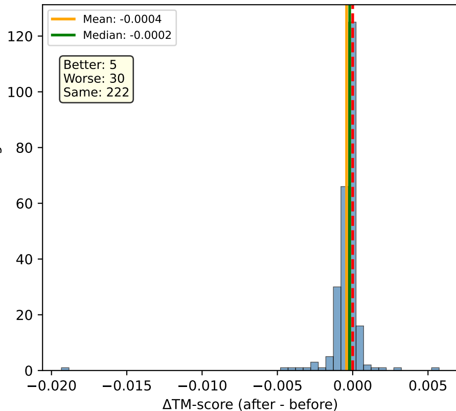
AF2: Built-in AMBER
