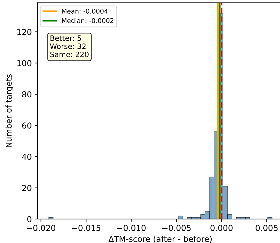
AF2: Standalone AMBER
