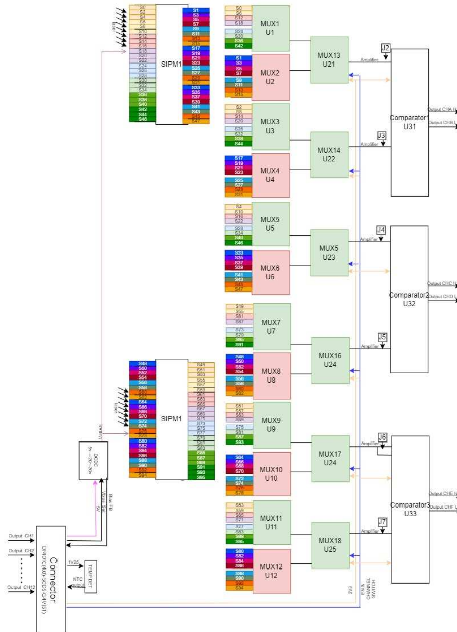
Robin-E lite Detector diagram
