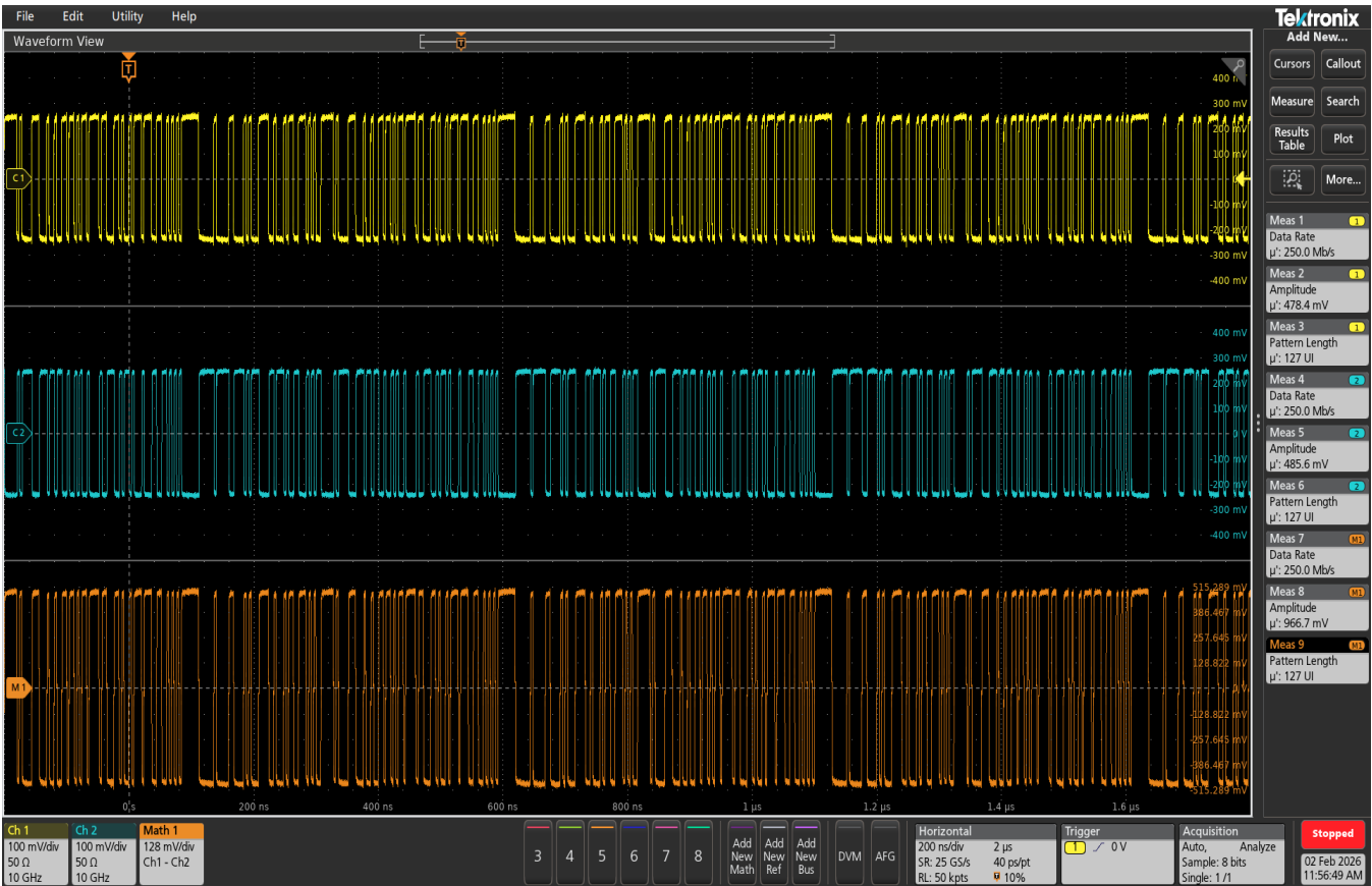
Test 1: prbs7_capture.png
