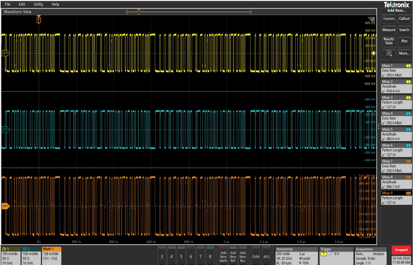
Test 7: prbs7_capture.png
