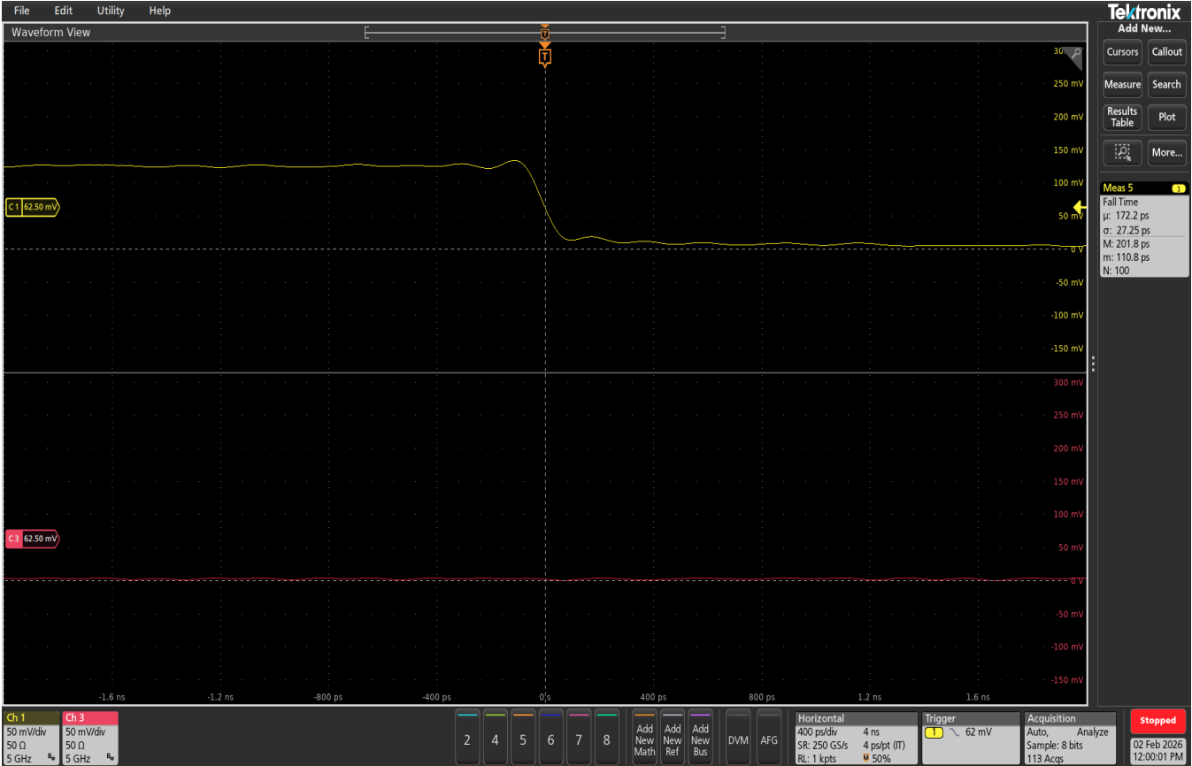
Test 5: fall_time_ch1.png
