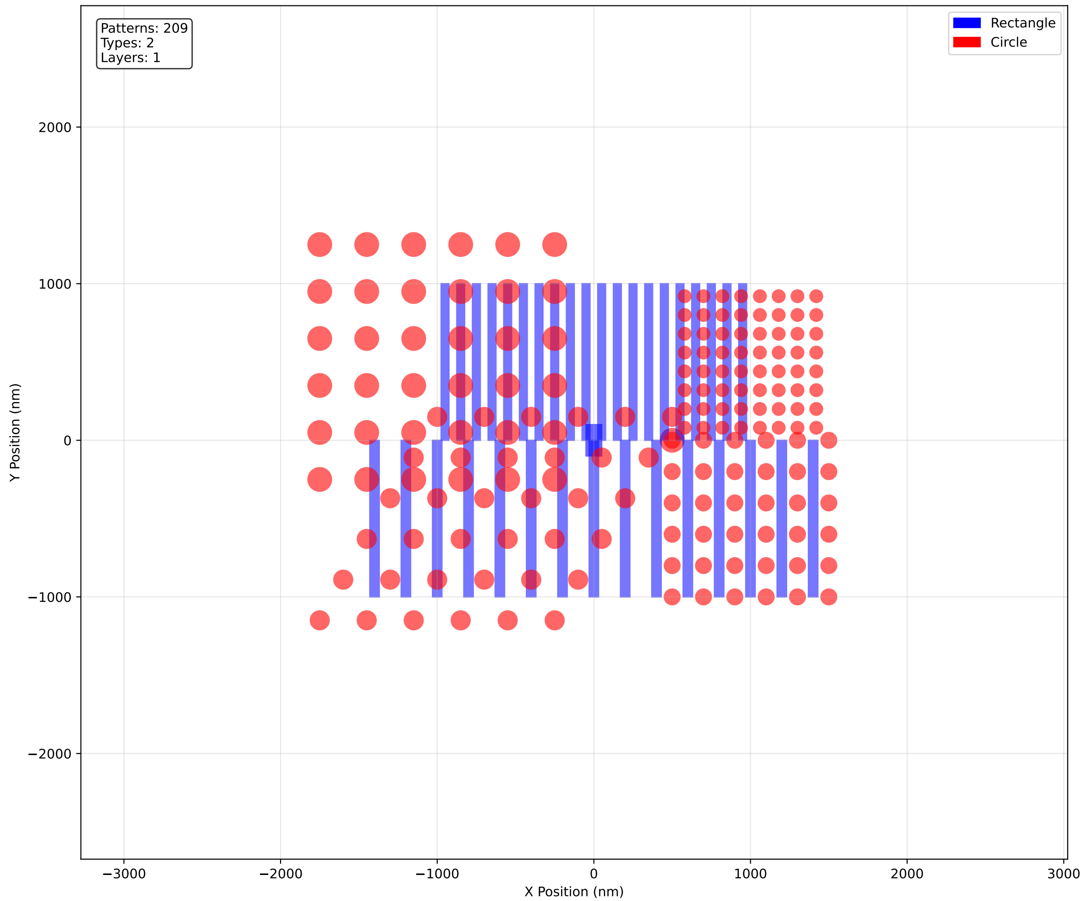
Advanced EBL Test Patterns
