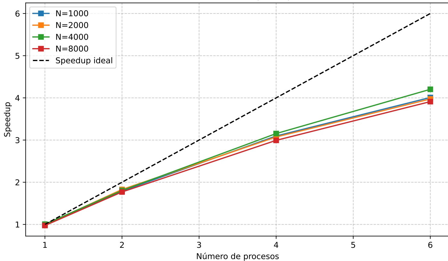
Matriz-vector: speedup
