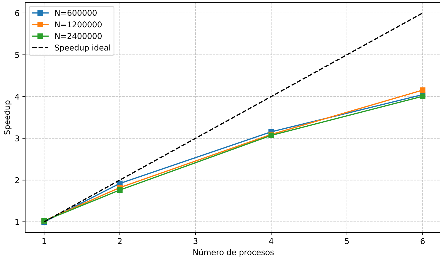
Odd-Even: speedup
