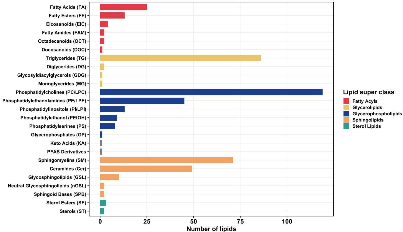
Identified lipids by class
