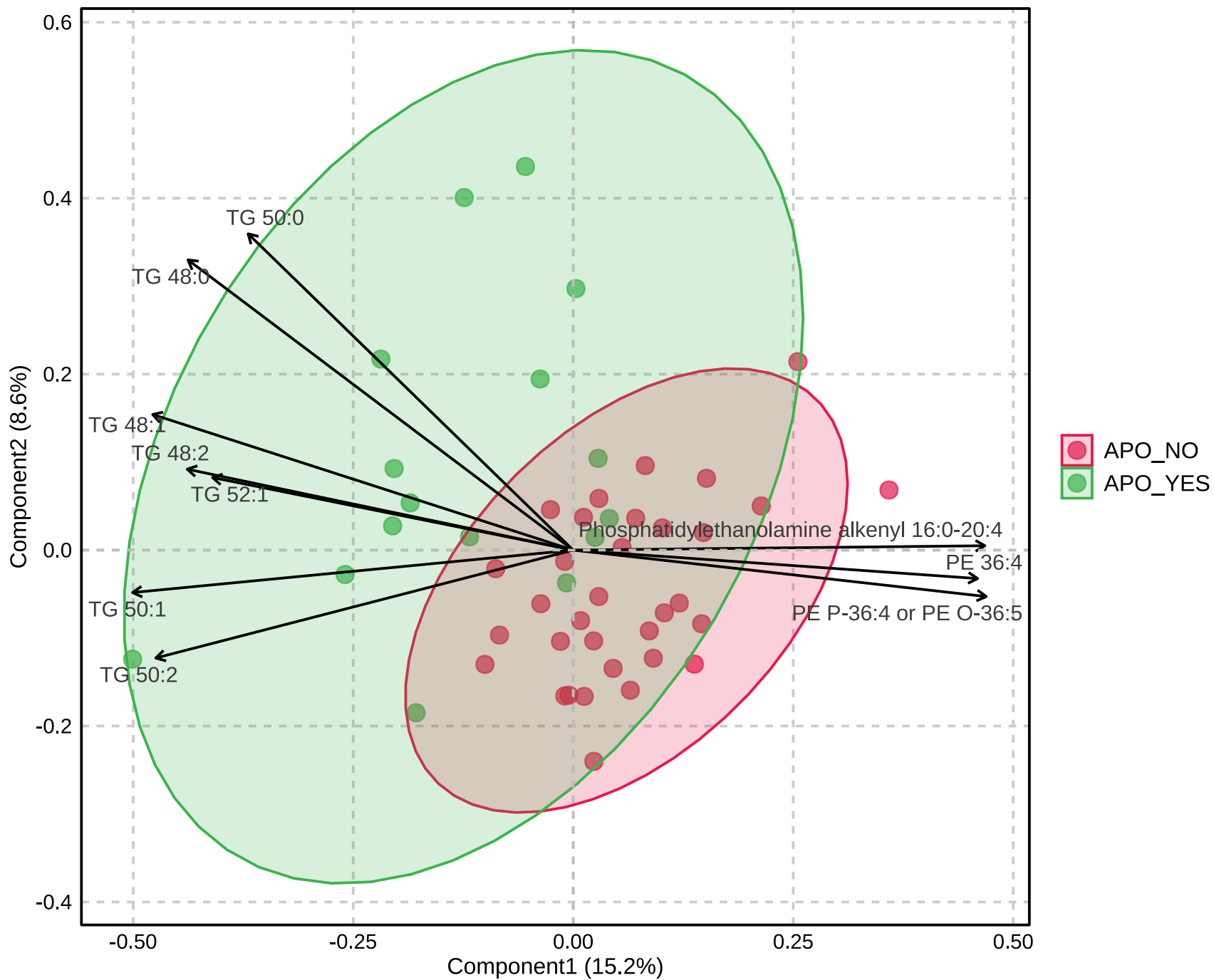
Biplot
