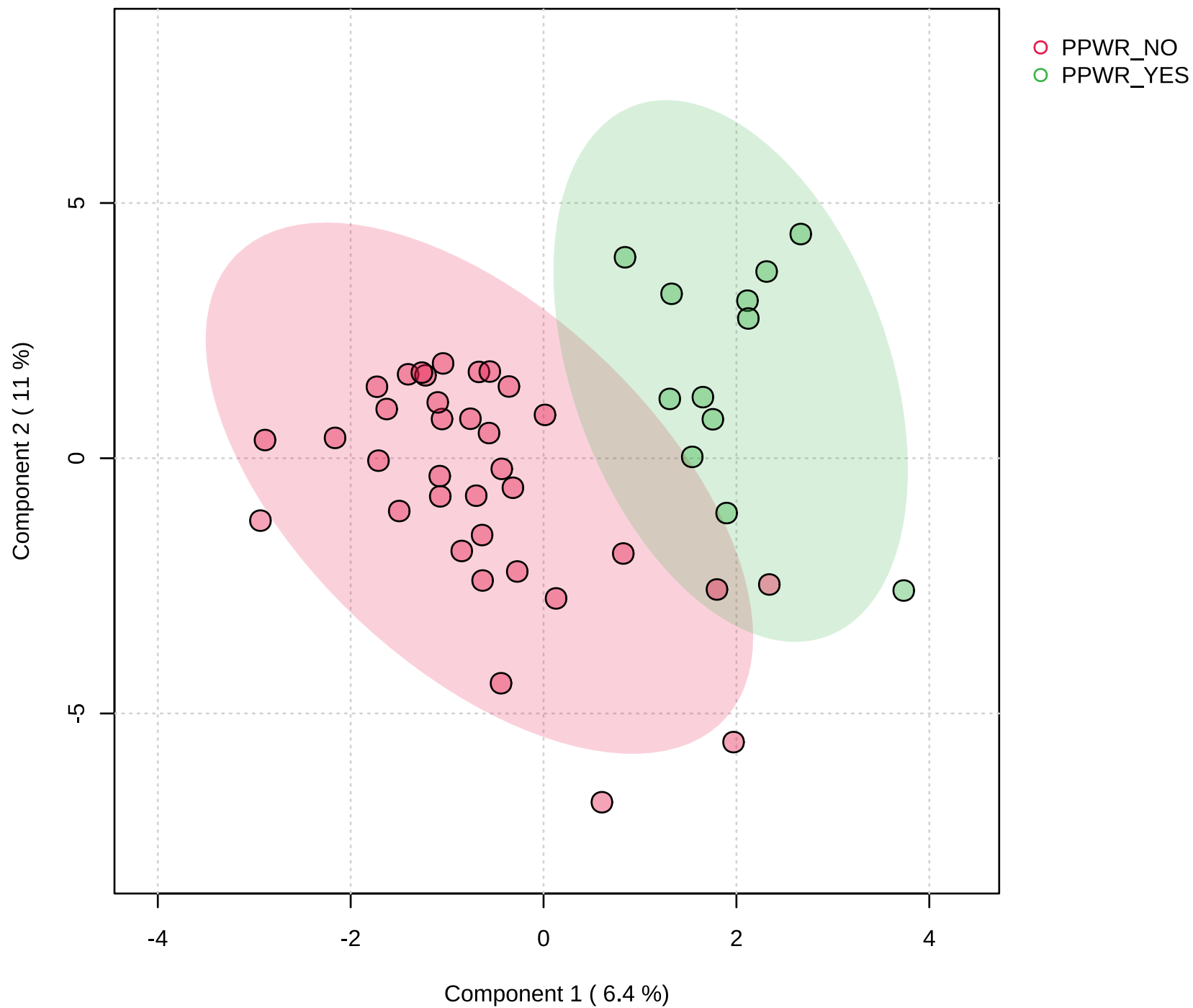
Scores Plot
