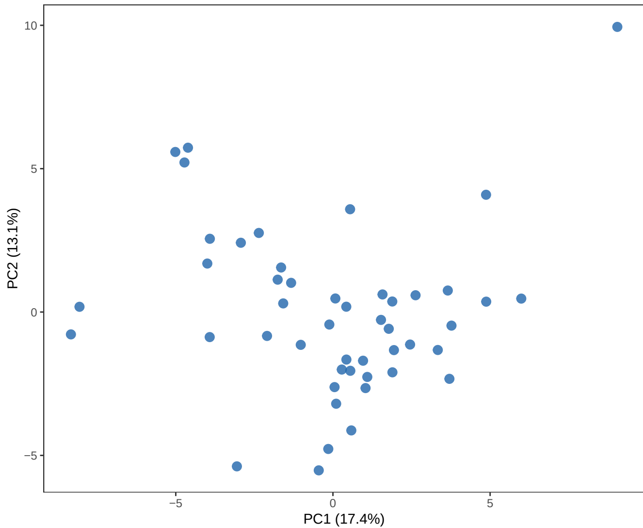
Baseline – PCA (post-normalization)
