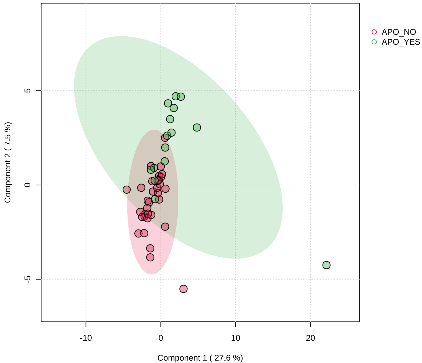
Scores Plot
