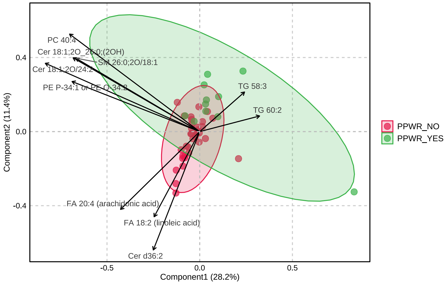
Biplot
