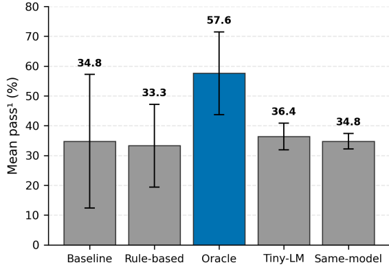
Figure 1: Mean pass 1 ( \pm 1 std across 3 seeds) for five planning conditions on 22 complex retail tasks. Oracle planning (+22.7 pp) is the only condition with meaningful improvement. Automated planners also reduce cross-seed variance (narrowing error bars).
