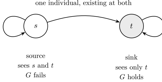
Figure 2: The S4 chain of \mathbf{R\_chain} , drawn as source s = \text{false} and sink t = \text{true} . Reflexive, transitive, and not symmetric. The domain has one element, and existence is true at both worlds. Under \mathbf{chainP} , a God-like being exists at the sink only, so at the source a God-like being is possible and not necessary. Literal \text{Ax1Gen} has no model on this frame. Both reconstructions do.
