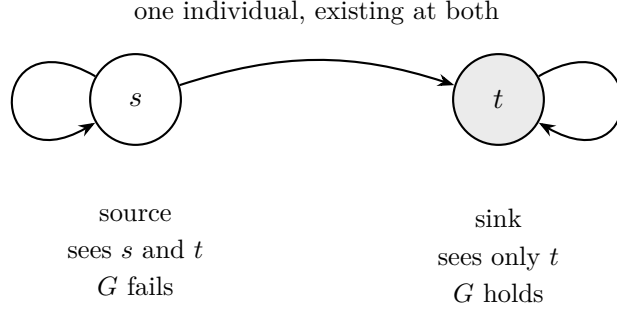
Figure 2: The S4 chain of R\_chain , drawn as source s = \text{false} and sink t = \text{true} . Reflexive, transitive, and not symmetric. The domain has one element, and existence is true at both worlds. Under chainP , a God-like being exists at the sink only, so at the source a God-like being is possible and not necessary. Literal Ax1Gen has no model on this frame. Both reconstructions do.
